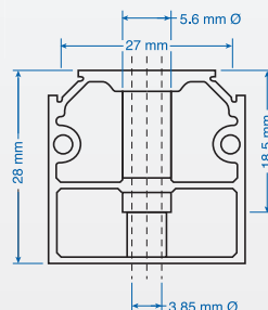
Mounting Section Dimensions EPCMB4
