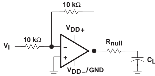
Figure 54. Series-Resistance Circuit
