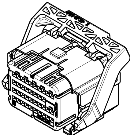
KEYING OPTION "G" SHOWN SEE SHEET 2 FOR BILL OF MATERIALS AND SHEET 3 FOR PIN-OUT CHARTS
