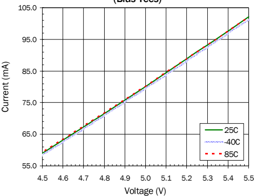
Current versus Voltage Over Temperature (Bias Tees)
