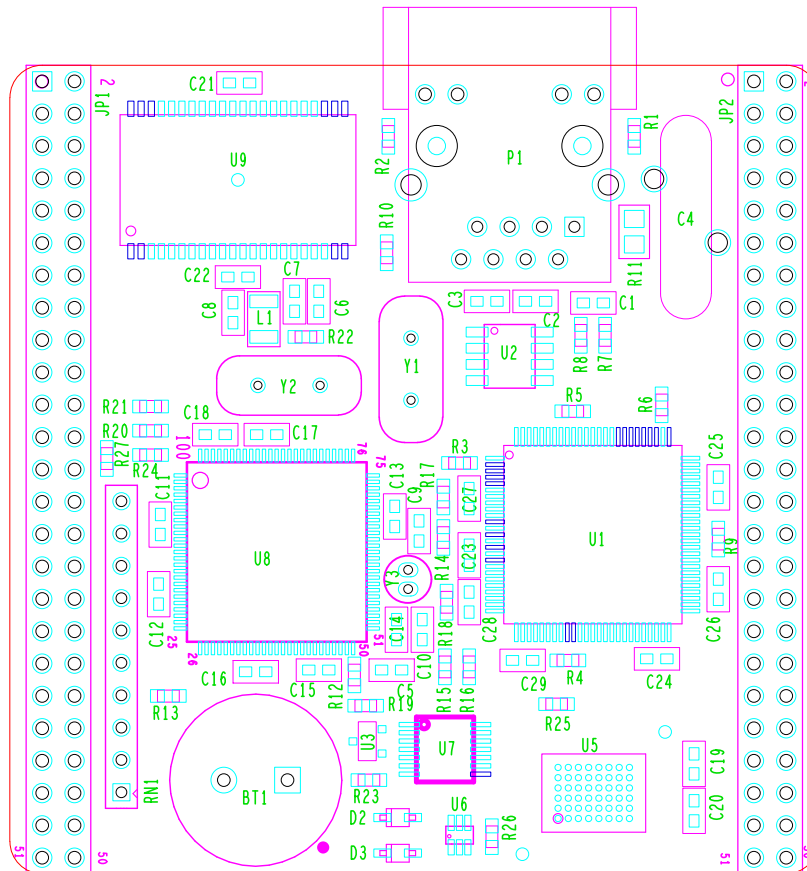
Figure 5. Top View
