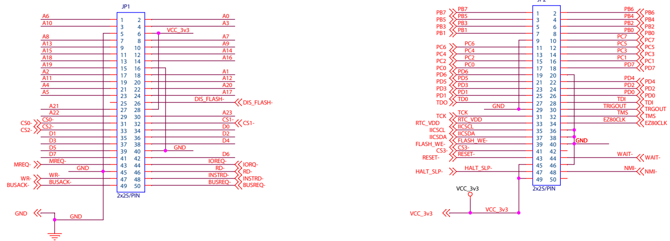
Figure 11. eZ80L92 Module Schematic Diagram, #4 of 4: Interfaces
