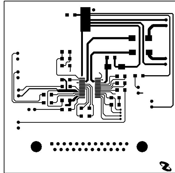
Figure 32. Top Layer
