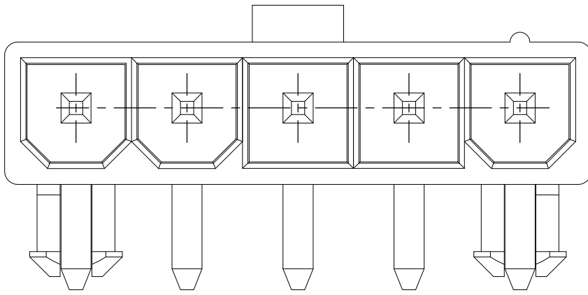
2029154-5 MATING FACE
