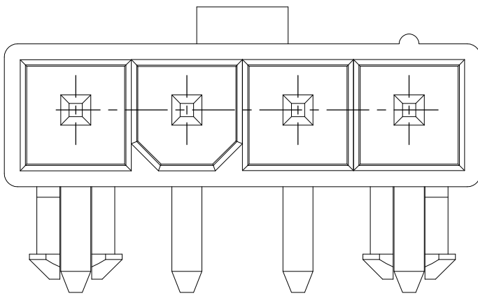
2029154-4 MATING FACE
