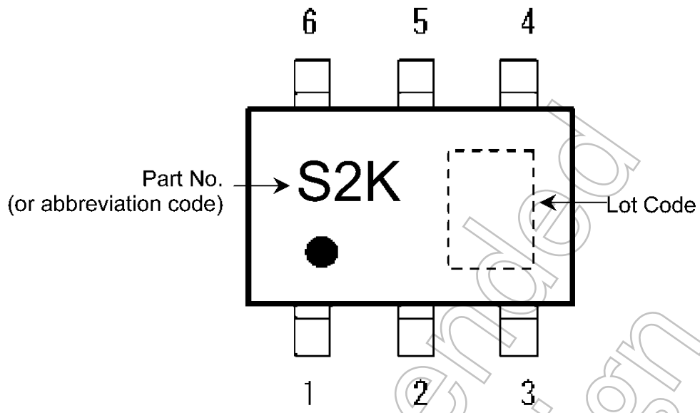
Fig. 7.1 Marking
