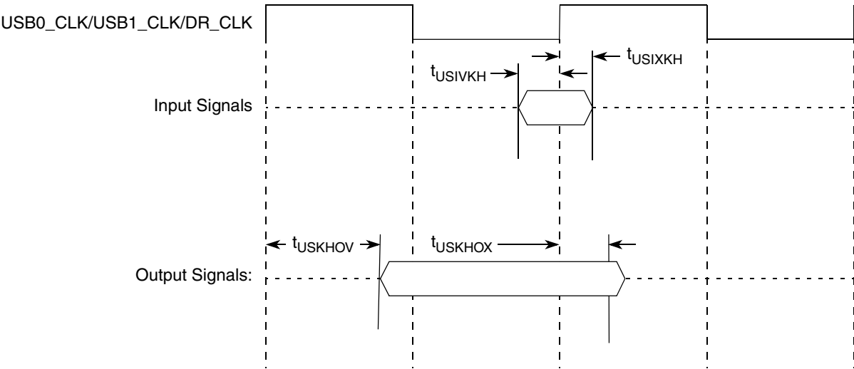
Figure 20. USB Signals
