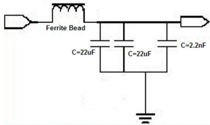
Figure 57. \text{XCOREV}_{\text{DD}} and \text{XPADV}_{\text{DD}} Power Supply Filter Circuit
