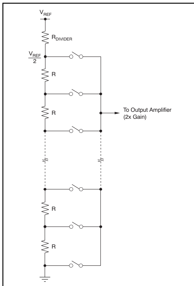
Figure 93. Resistor String
