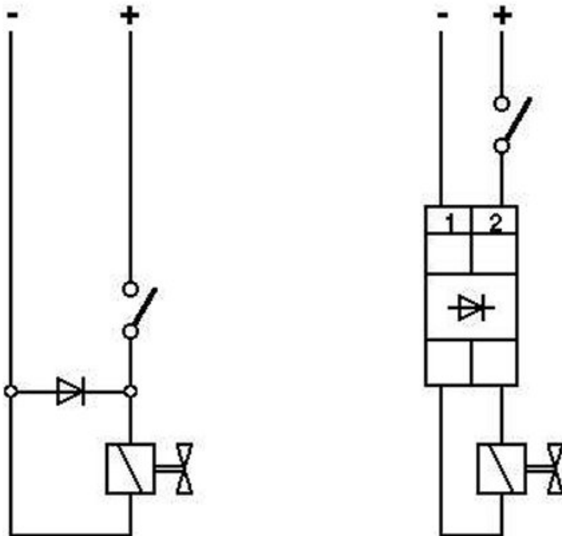
Circuit diagram
