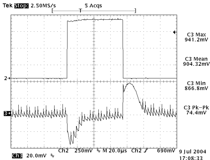
Figure 19: Typical transient response to step load change at 10A/μS from 50% to 75% and 75% to 50% of I_{o\_max} at 12Vin, 0.9V out
