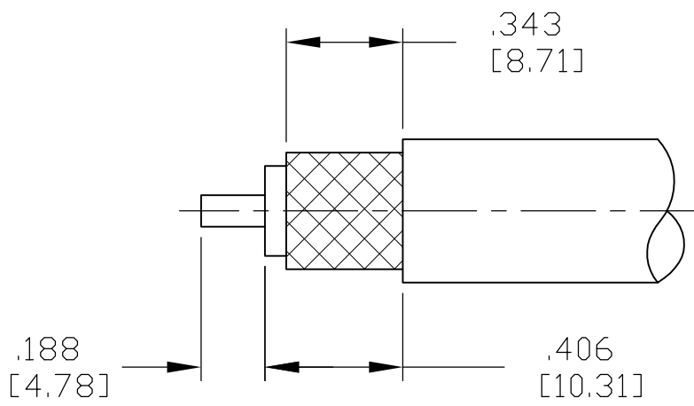
RECOMMENDED STRIP LENGTH SCALE 2:1
