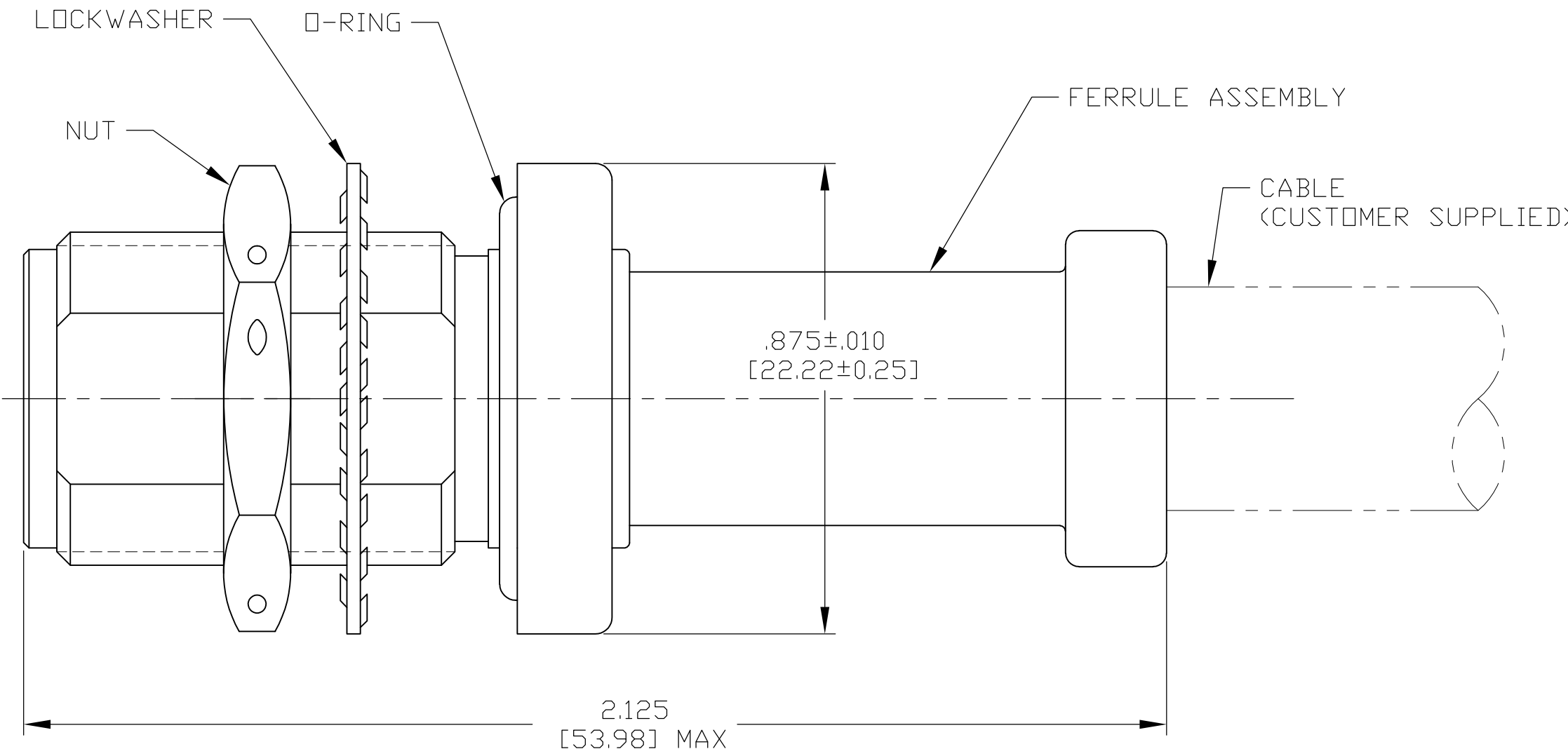
ASSEMBLED VIEW
