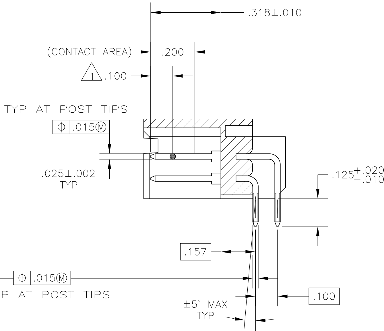
SECTION X-X
