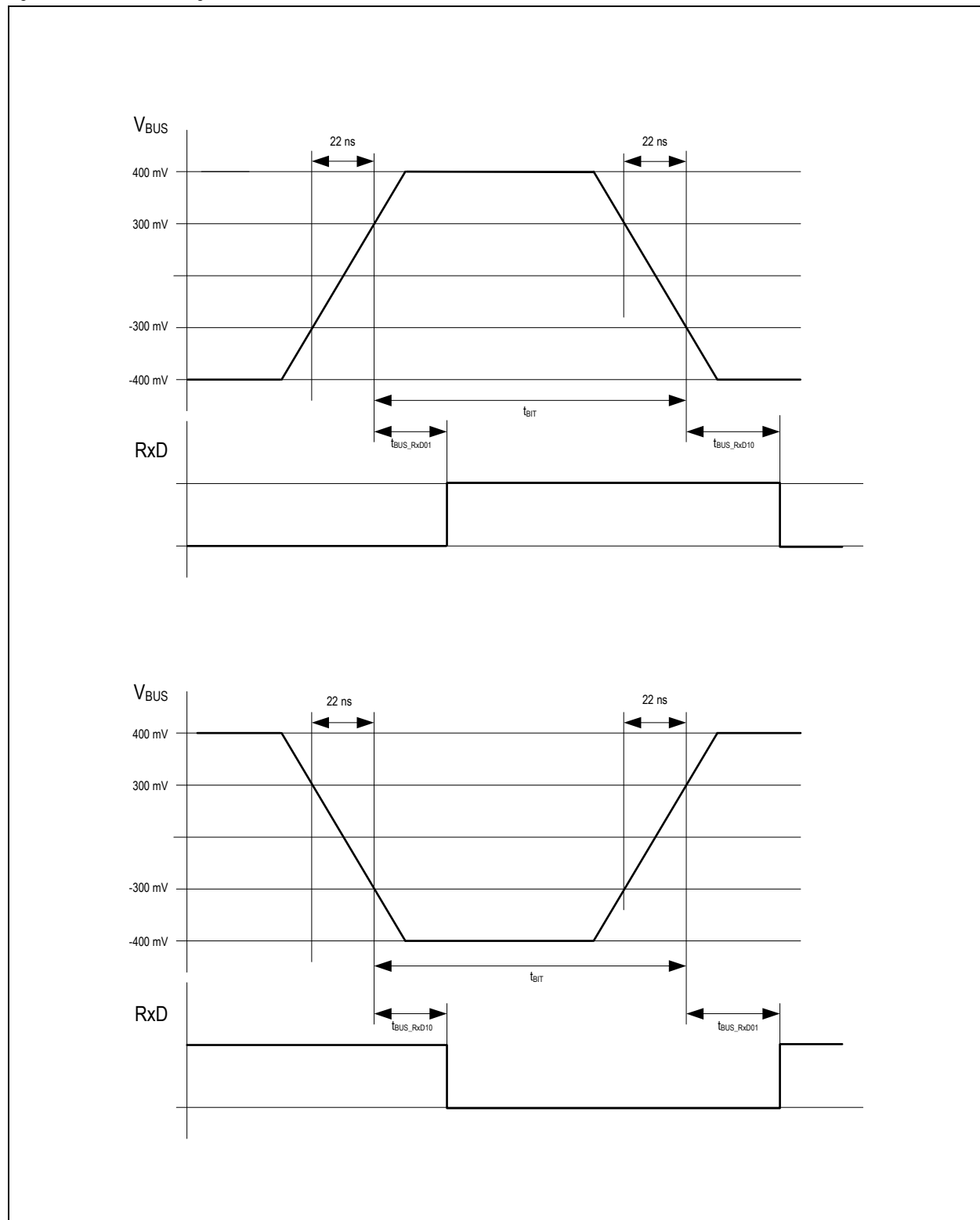
Figure 13. Receiver Test Signal
