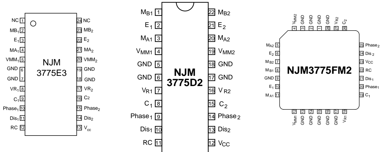
Figure 2. Pin configurations
