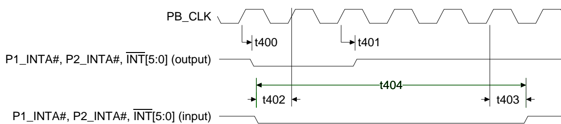
Figure 38: Interrupt Timing
