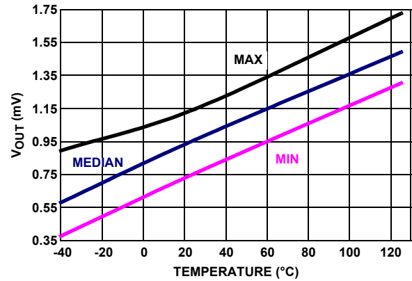
FIGURE 34. V_{OUT} LOW vs TEMPERATURE, V_+, V_- = \pm 2.5V, R_L = 100k
