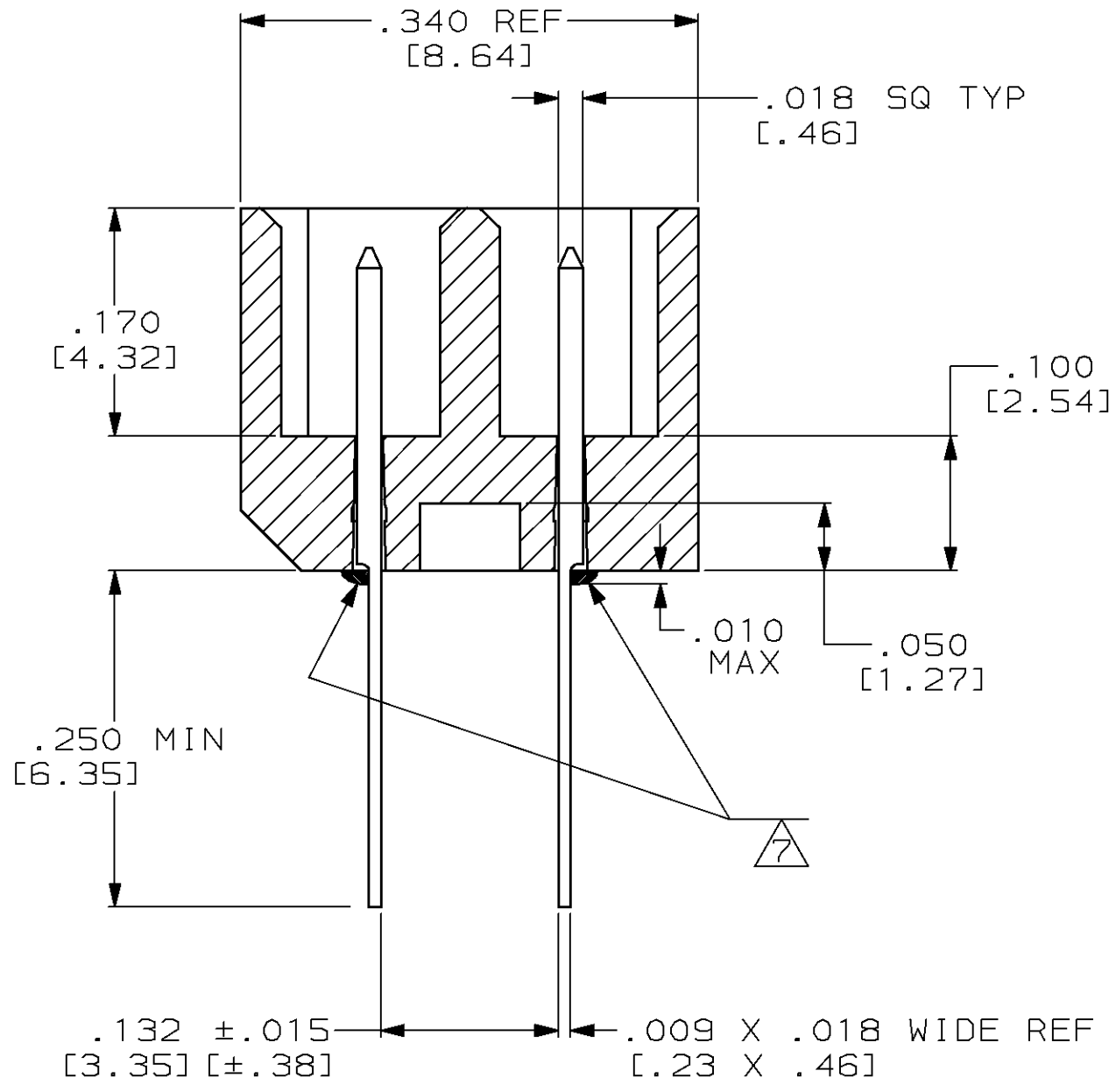
SECTION X-X SCALE 8:1
