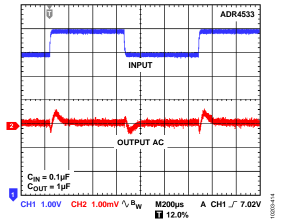
Figure 60. ADR4533 Line Transient Response
