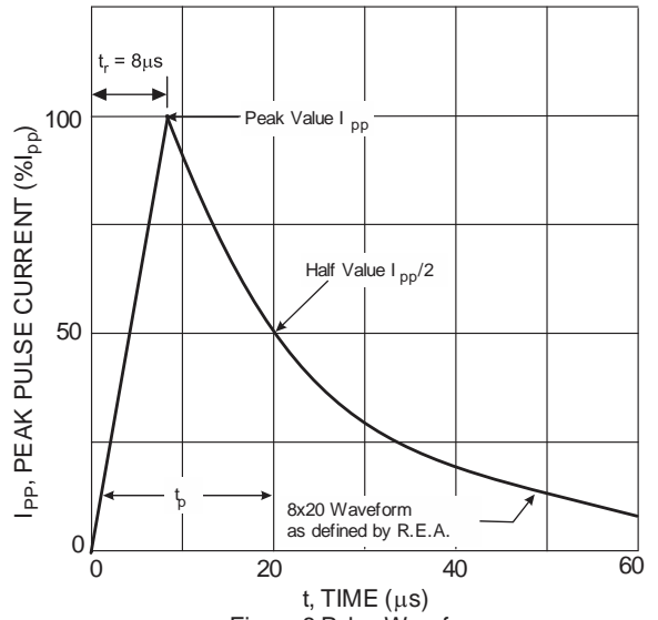
Figure 8 Pulse Waveform
