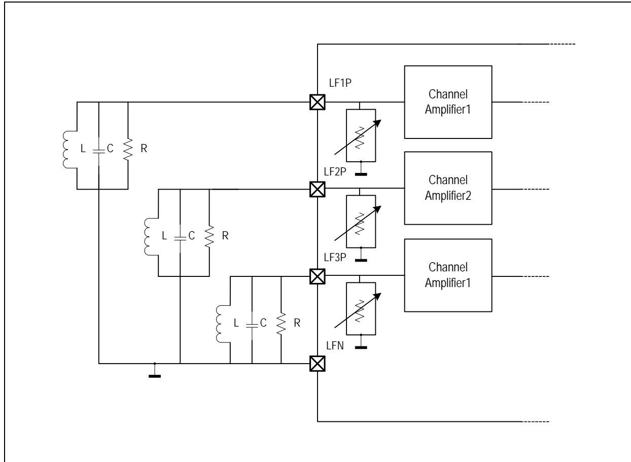
Figure 19. Antenna Damper
