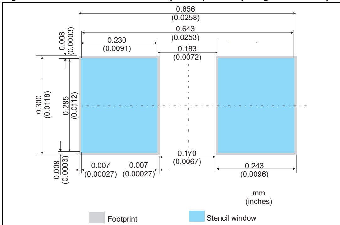
Figure 14. Recommended stencil window position, stencil opening thickness: 80 µm
