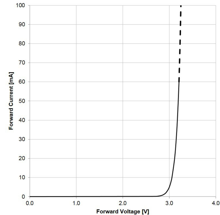
F3 Forward Current vs. Forward Voltage:
