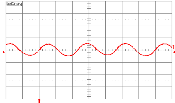
Figure 13. Input reflected ripple-current, i_c (200 mA/div.), measured at input terminals at full rated load current and V_{in} = 48 V. Refer to Figure 11 for test setup. Time scale: 1 \mu s/div.
