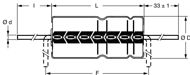
Form AA: Axial in box Case ∅ D x L = 10 mm x 30 mm to 21 mm x 38 mm
