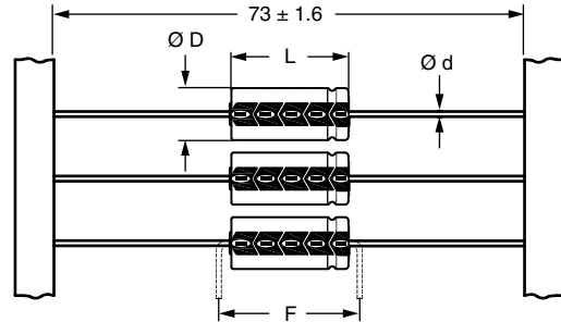
Form BR: Taped on reel Case ∅ D x L = 6.5 mm x 18 mm to 15 mm x 30 mm Form BA: Taped in box (ammpack) Case ∅ D x L = 6.5 mm x 18 mm to 10 mm x 25 mm
