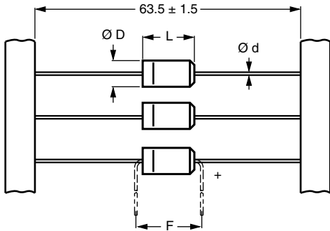
Form BR: Taped on reel Form BA: Taped in box (ammpack) Case ∅ D x L = 6.3 mm x 12.7 mm to 7.7 mm x 12.7 mm
