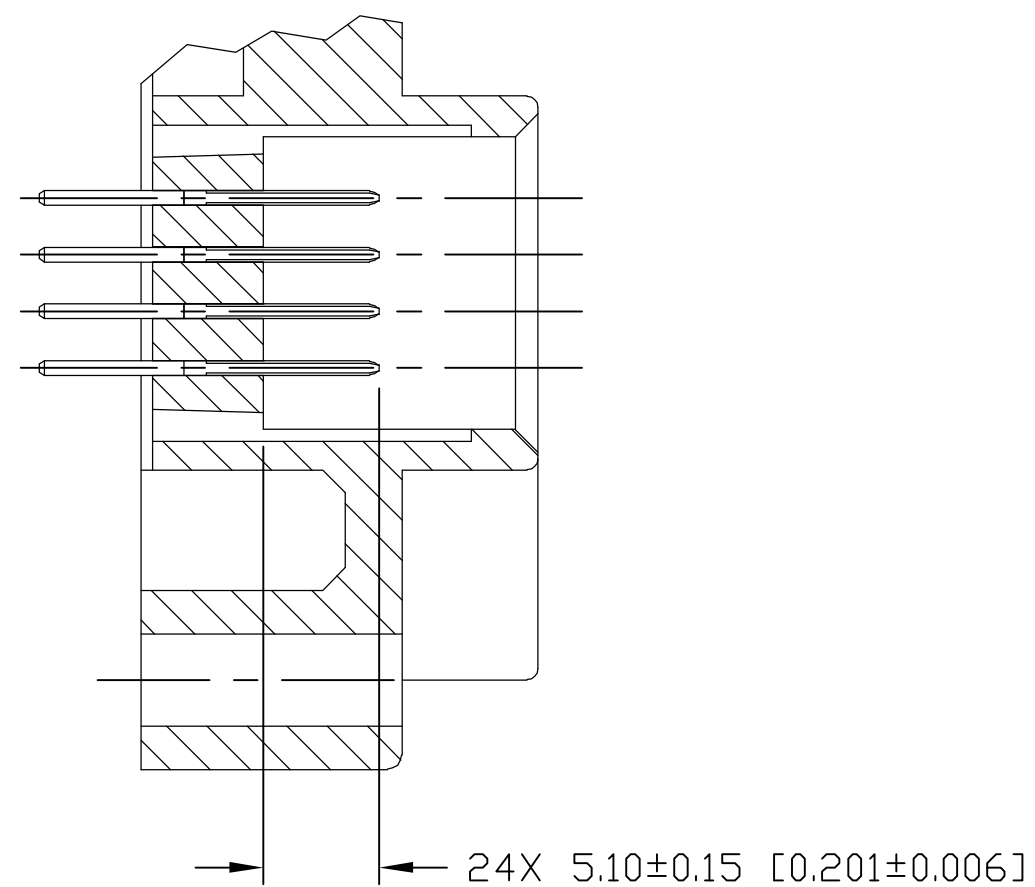
DETAIL F
