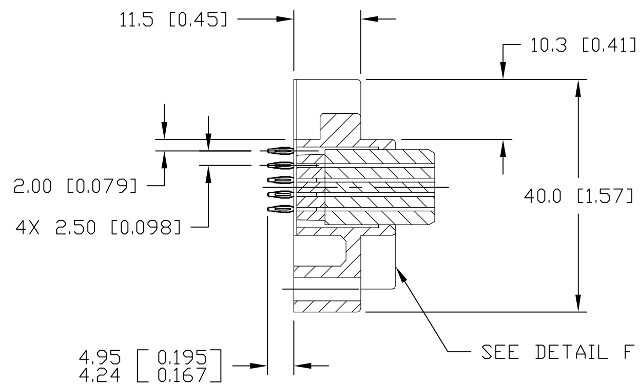
SECTION E-E
