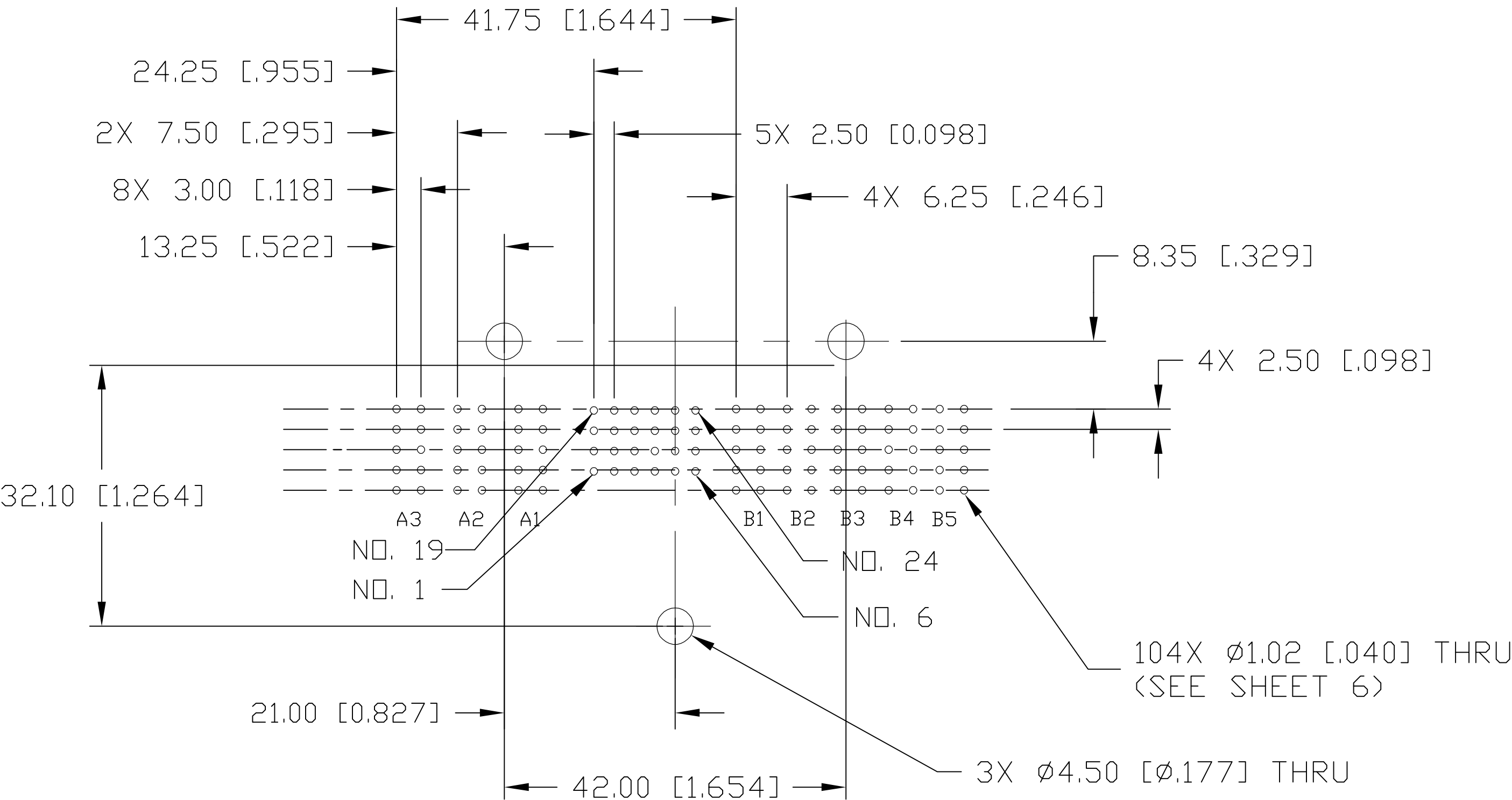
SUGGESTED PC BOARD LAYOUT VIEW FROM CONNECTOR MOUNTING SIDE
