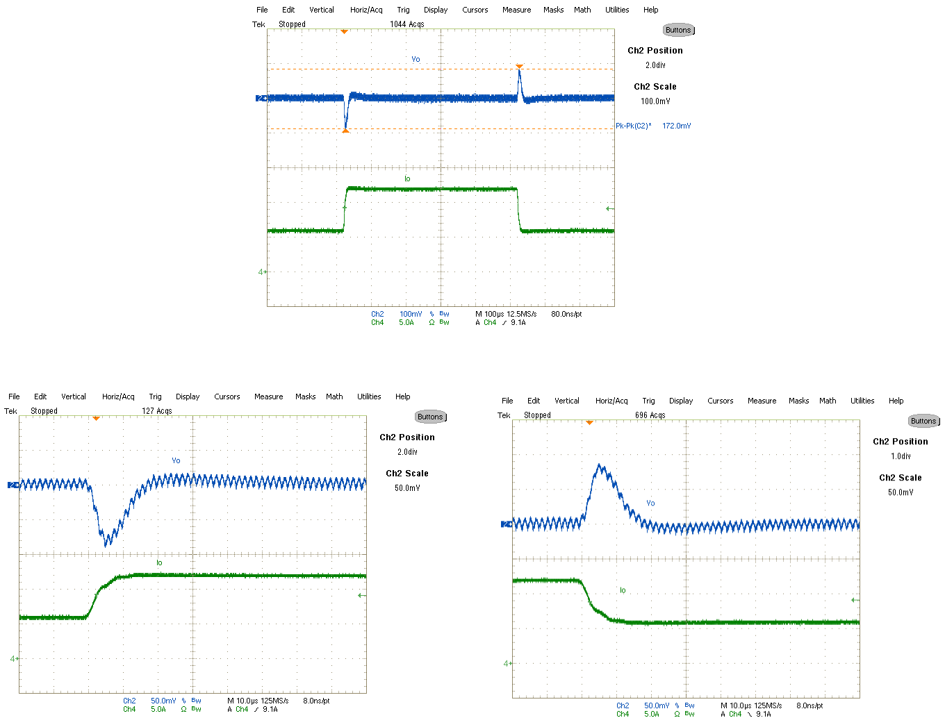
Fig. 13: Transient Response, 6A to 12A step 2.5A/\mu s Ch_2: V_{out} , Ch_4: I_{out}
