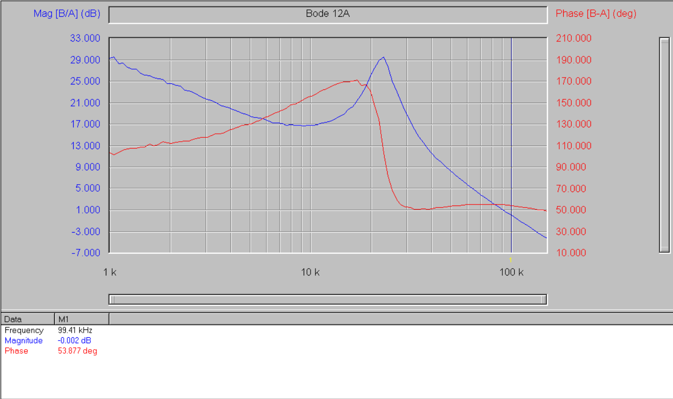
Fig. 14: Bode Plot at 12A load shows a bandwidth of 99kHz and phase margin of 54 degrees
