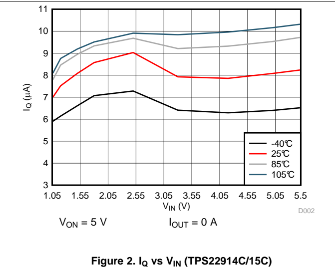
Figure 2. I_Q vs V_{IN} (TPS22914C/15C)
