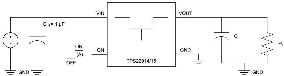
Figure 33. Test Circuit
