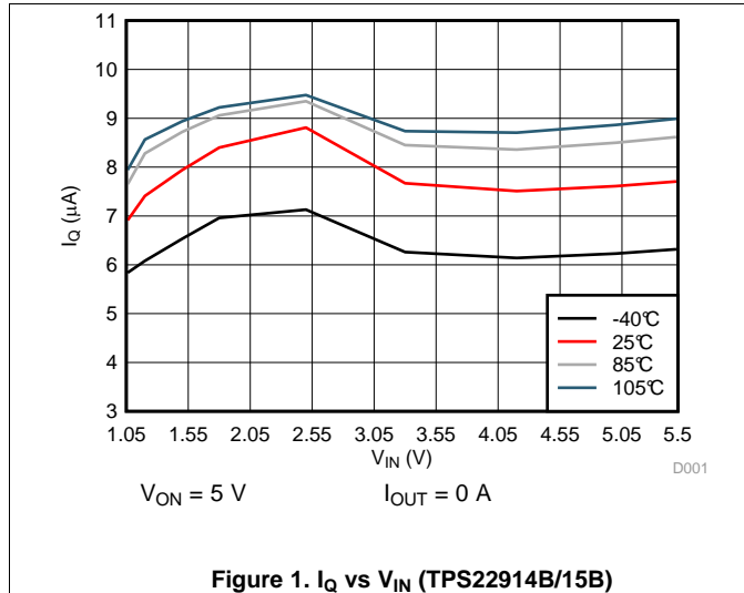
Figure 1. I_Q vs V_{IN} (TPS22914B/15B)
