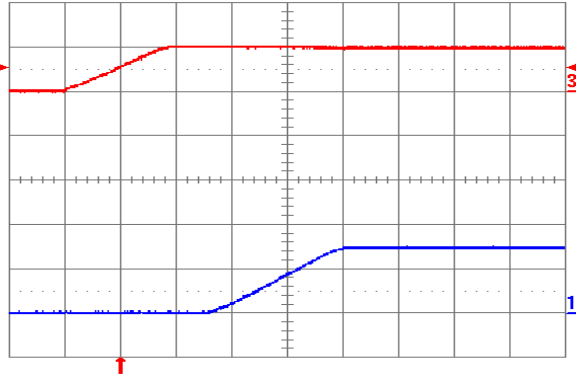
Fig. 1.5V.4: Turn-on transient for V_{out} = 1.5\text{ V} with application of V_{in} at full rated load current (resistive) and 100\ \mu\text{F} external capacitance at V_{in} = 5\text{ V} . Top trace: V_{in} ( 5\text{ V/div.} ); Bottom trace: output voltage ( 1\text{ V/div.} ); Time scale: 2\text{ ms/div.}
