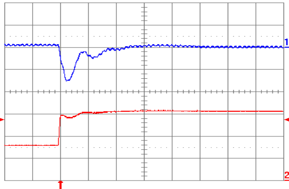
Fig. 1.5V.6: Output voltage response for V_{out} = 1.5\text{ V} to positive load current step change from 8\text{ A} to 16\text{ A} with slew rate of 5\text{ A}/\mu\text{s} at V_{in} = 5\text{ V} . Top trace: output voltage ( 100\text{ mV/div.} ); Bottom trace: load current ( 5\text{ A/div.} ). C_o = 100\ \mu\text{F} ceramic + 1\ \mu\text{F} ceramic. Time scale: 20\ \mu\text{s/div.}
