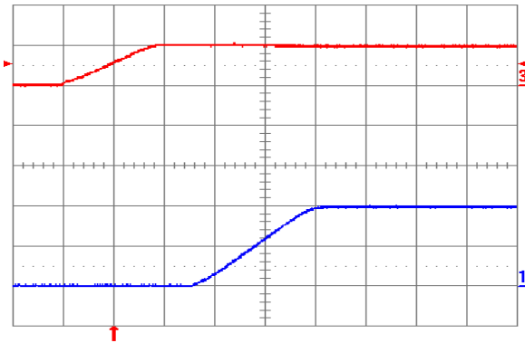
Fig. 2.0V.4: Turn-on transient for V_{out} = 2.0 V with application of V_{in} at full rated load current (resistive) and 100 \mu F external capacitance at V_{in} = 5 V. Top trace: V_{in} (5 V/div.); Bottom trace: output voltage (1 V/div.); Time scale: 2 ms/div.
