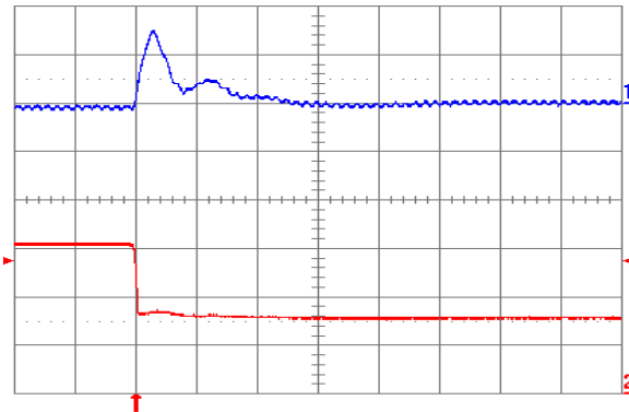
Fig. 1.5V.7: Output voltage response for V_{out} = 1.5\text{ V} to negative load current step change from 16\text{ A} to 8\text{ A} with slew rate of -5\text{ A}/\mu\text{s} at V_{in} = 5\text{ V} . Top trace: output voltage ( 100\text{ mV/div.} ); Bottom trace: load current ( 5\text{ A/div.} ). C_o = 100\ \mu\text{F} ceramic + 1\ \mu\text{F} ceramic. Time scale: 20\ \mu\text{s/div.}
