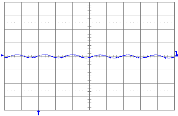
Fig. 1.0V.5: Output voltage ripple (20 mV/div.) at full rated load current into a resistive load with external capacitance 100\text{ }\mu\text{F} ceramic + 1\text{ }\mu\text{F} ceramic and V_{in} = 5\text{ V} for V_{out} = 1.0\text{ V} . Time scale: 2\text{ }\mu\text{s}/\text{div} .
