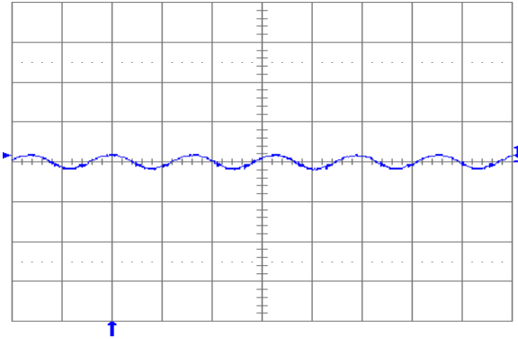
Fig. 1.5V.5: Output voltage ripple ( 20\text{ mV/div.} ) at full rated load current into a resistive load with external capacitance 100\ \mu\text{F} ceramic + 1\ \mu\text{F} ceramic and V_{in} = 5\text{ V} for V_{out} = 1.5\text{ V} . Time scale: 2\ \mu\text{s/div.}
