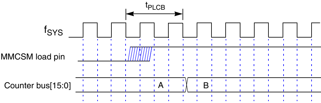
Figure G-41 MMCSM Load Pin to Counter Bus Reload Timing Diagram
