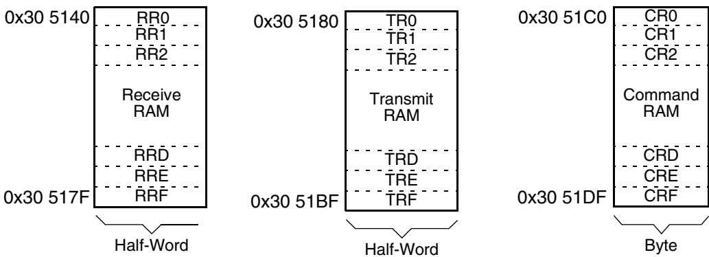
Figure 14-5 QSPI RAM
