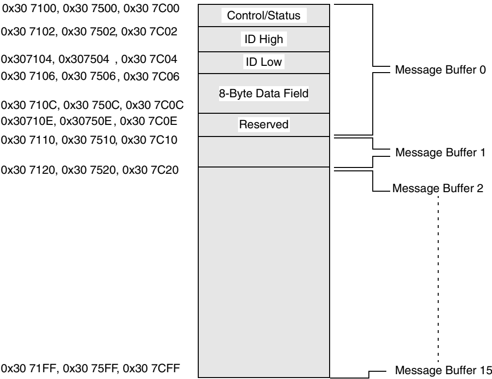
Figure 16-6 TouCAN Message Buffer Memory Map
