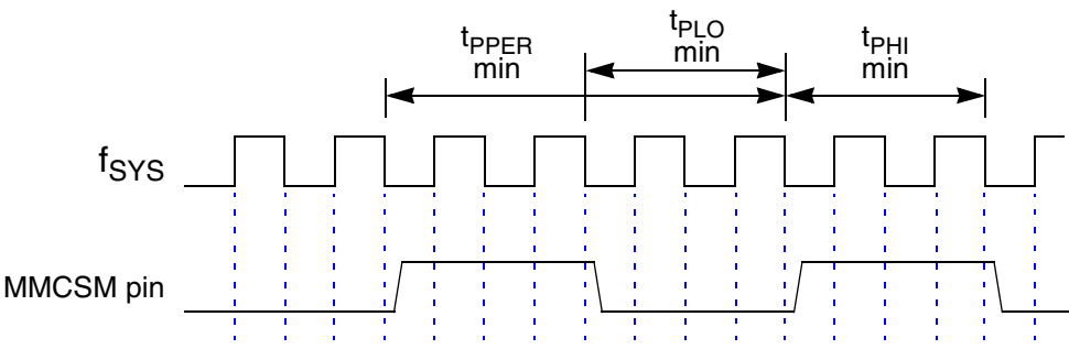
Figure G-39 MMCSM Minimum Input Pin (Either Load or Clock) Timing Diagram
