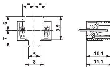
Dimensional drawing
