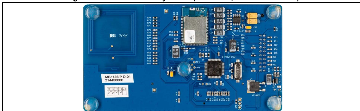
Figure 2. M24SR Discovery board (back side, Premium edition)
