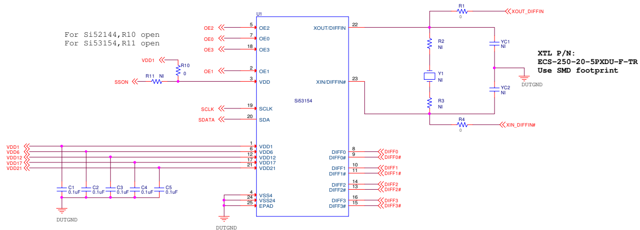
Figure 2. QFN-24 Device Connection
