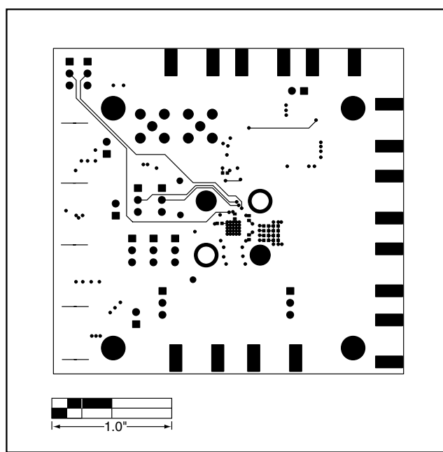
Figure 5. MAX3670 EV Kit PC Board Layout—Solder Side
