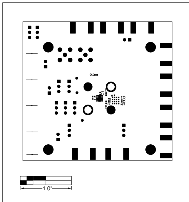
Figure 3. MAX3670 EV Kit Component Placement Guide—Solder Side
