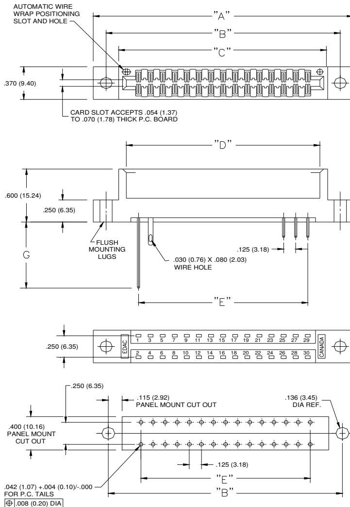
CONNECTOR MOUNTING PATTERN
