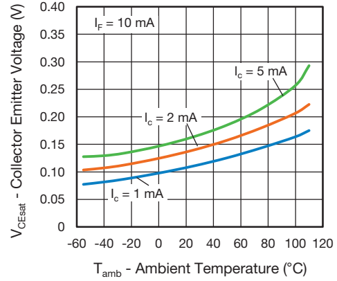
Fig. 11 - Collector Emitter Voltage vs. Ambient Temperature (saturated)
