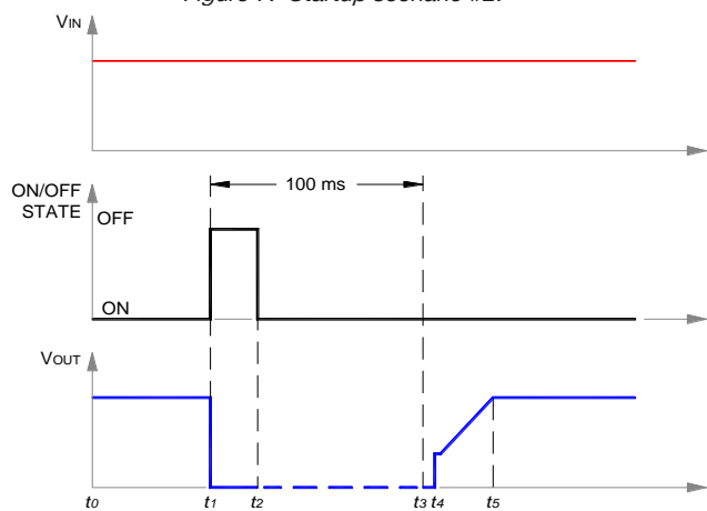
Figure 8. Startup scenario #3.
