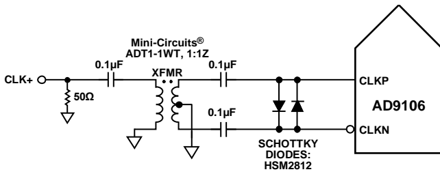
Figure 41. Transformer Coupled Clock
