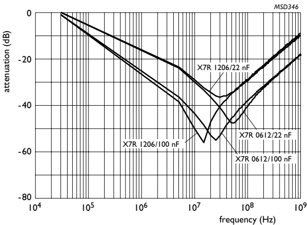
Fig.2 Comparison of transmission characteristics of standard MLCCs and Yageo's Phycomp branded low-inductance MLCCs
