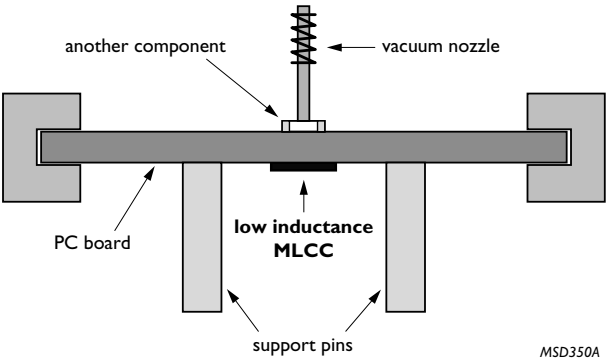
Fig.6 Precautions when handling substrate
