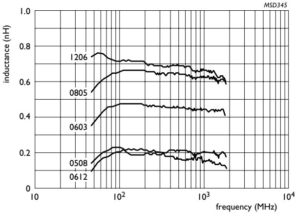
Fig.1 ESL measurements of X7R 100 nF MLCCs
