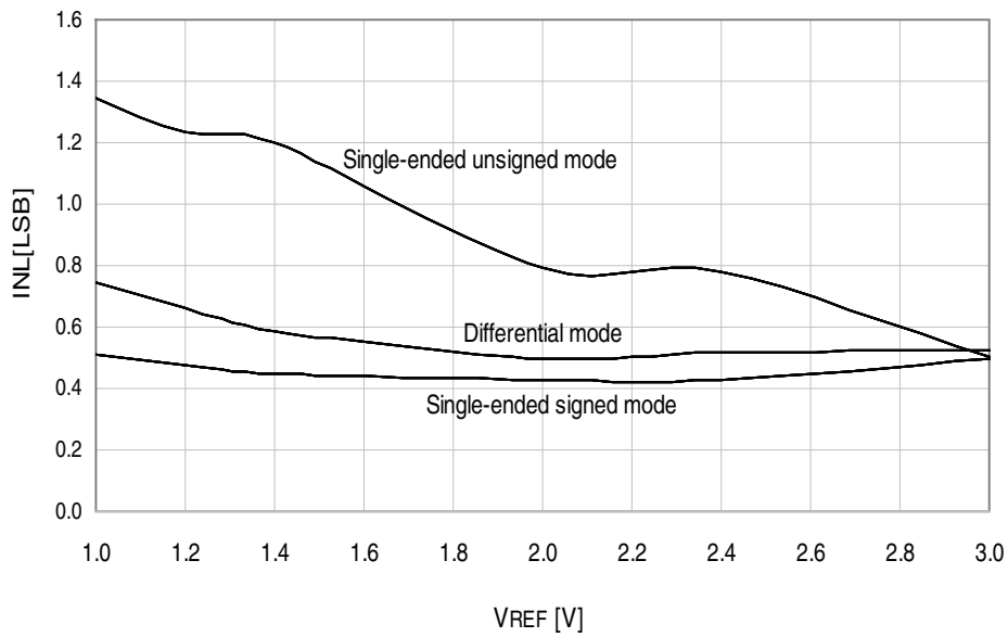
Figure 34-242. INL Error vs. External V_{REF}
