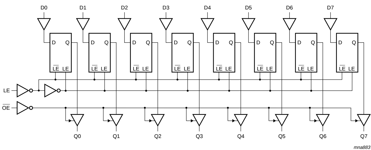
Fig 5. Logic diagram
