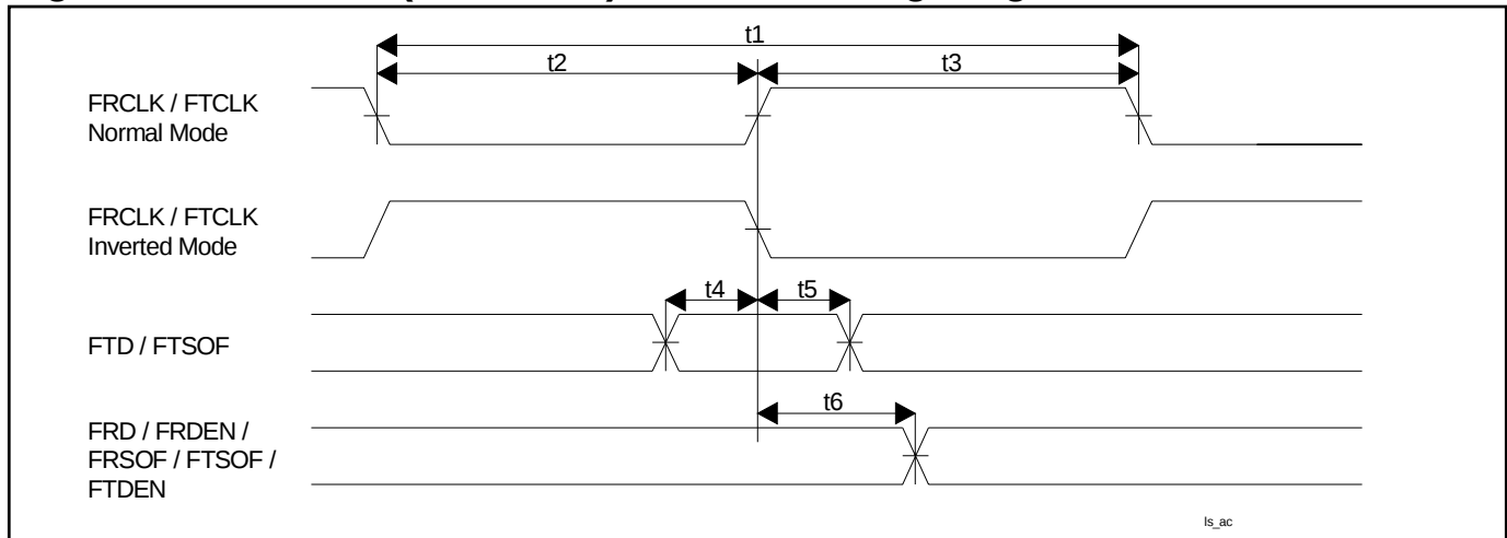
Figure 13-3. Framer (T3 and E3) Port AC Timing Diagram
