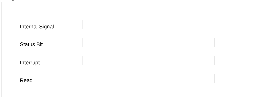
Figure 4-1. Event Status Bit
