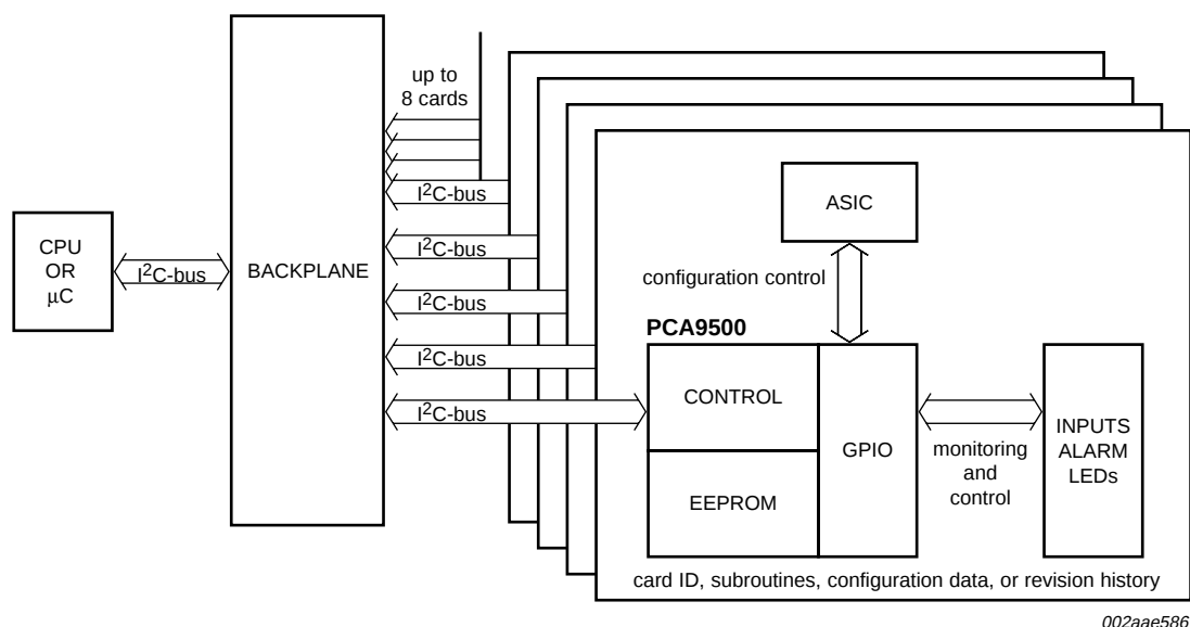
Fig 19. PCA9500 used as interface for board configuration
