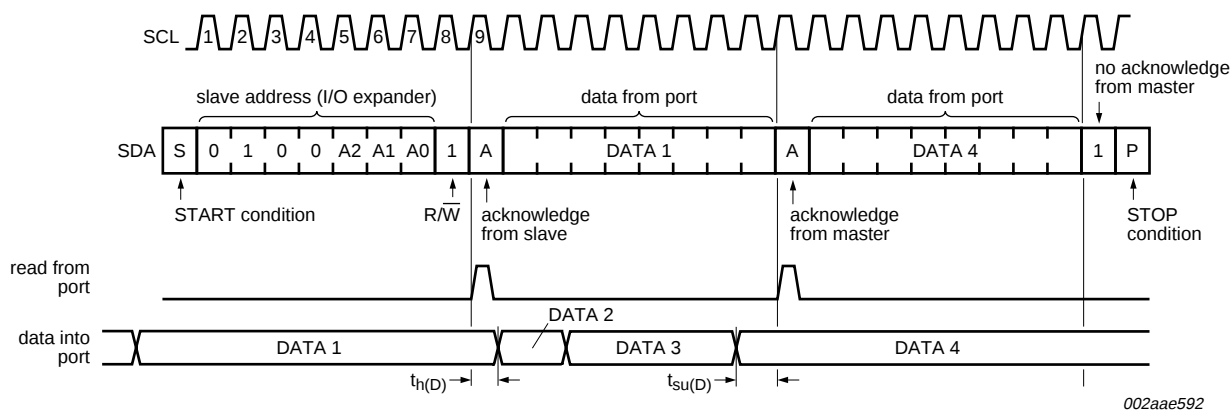
Fig 8. I/O Read mode (input)
