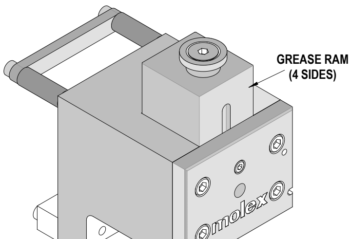
Figure 3-1 RAM LUBRICATION
