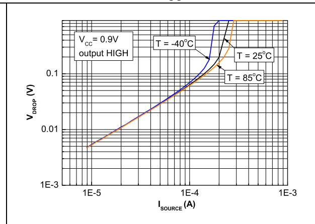
Figure 37. Output voltage drop vs. source current at V_{CC} = 0.9\text{ V}
