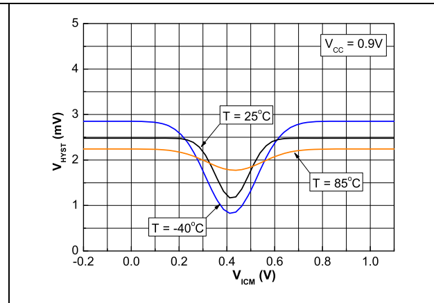
Figure 35. Input voltage hysteresis vs. input common mode voltage at V_{CC} = 0.9\text{ V}
