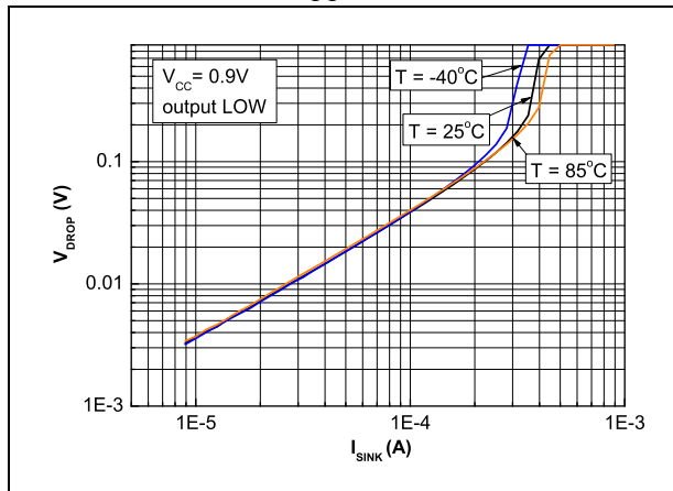
Figure 36. Output voltage drop vs. sink current at V_{CC} = 0.9\text{ V}
