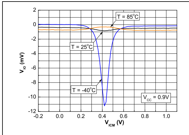
Figure 34. Input offset voltage vs. input common mode voltage at V_{CC} = 0.9\text{ V}
