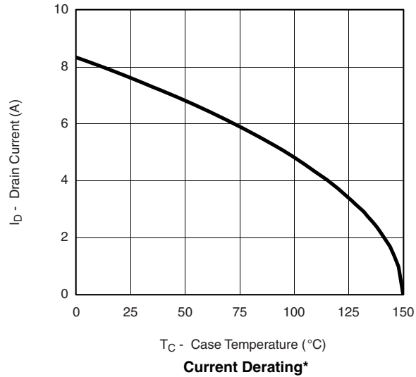
Current Derating*
