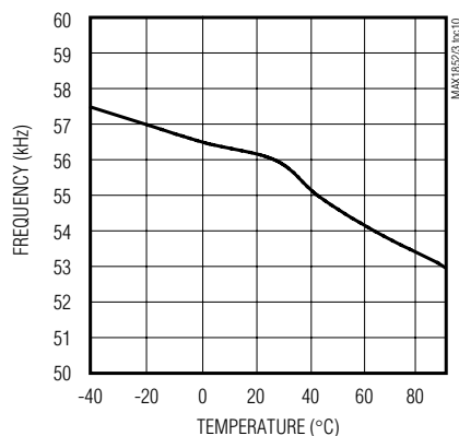
MAX1852 CHARGE-PUMP FREQUENCY vs. TEMPERATURE
