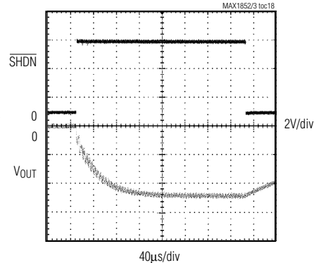
MAX1853 STARTUP FROM SHUTDOWN
