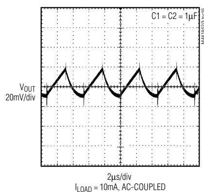
MAX1853 OUTPUT NOISE AND RIPPLE
