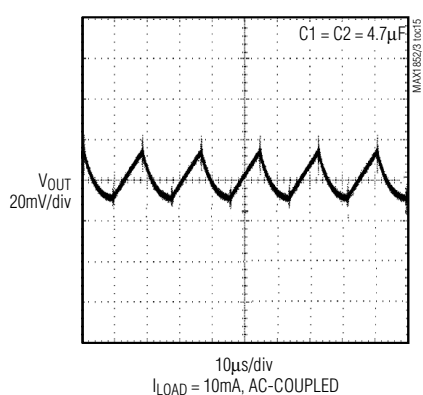
MAX1852 OUTPUT NOISE AND RIPPLE
