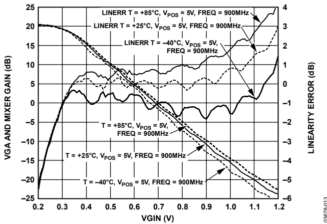
Figure 13. Mixer Gain and Linearity Error vs. VGIN, V_{POS} = 5V , F_{IF} = 900MHz , F_{BB} = 1MHz , Temperature = -40^{\circ}C , +25^{\circ}C , +85^{\circ}C
