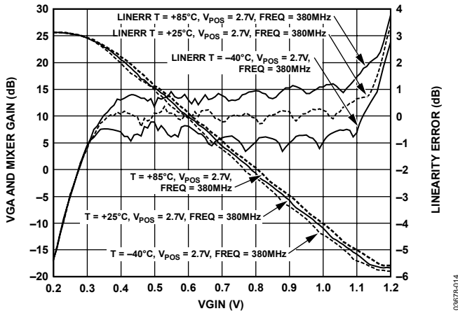
Figure 14. Mixer Gain and Linearity Error vs. VGIN, V_{POS} = 2.7V , F_{IF} = 380MHz , F_{BB} = 1MHz , Temperature = -40^{\circ}C , +25^{\circ}C , +85^{\circ}C
