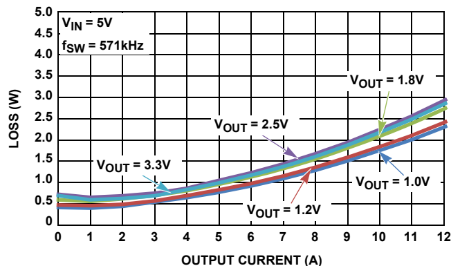
FIGURE 13. POWER LOSS CURVE, 5\text{V}_{\text{IN}} , FOR VARIOUS OUTPUT VOLTAGES LISTED
