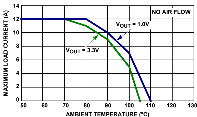
FIGURE 11. DERATING CURVE, 5\text{V}_{\text{IN}} , FOR VARIOUS OUTPUT VOLTAGES LISTED
