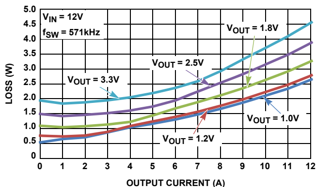
FIGURE 14. POWER LOSS CURVE, 12\text{V}_{\text{IN}} , FOR VARIOUS OUTPUT VOLTAGES LISTED
