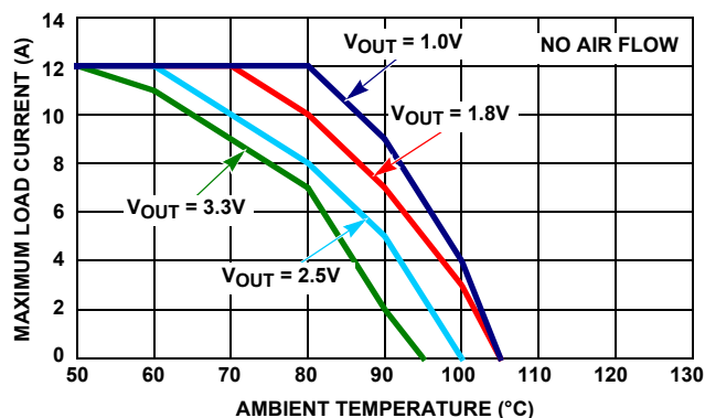
FIGURE 12. DERATING CURVE, 12\text{V}_{\text{IN}} , FOR VARIOUS OUTPUT VOLTAGES LISTED
